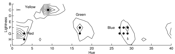
Figure 2. Contour plot of WCS best example choices, compared with best examples of English color terms.
